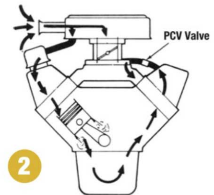
Typical PCV system configuration, PCV valve mounted on one valve cover with fresh air intake on opposite valve cover, shown above in Figure 2.
